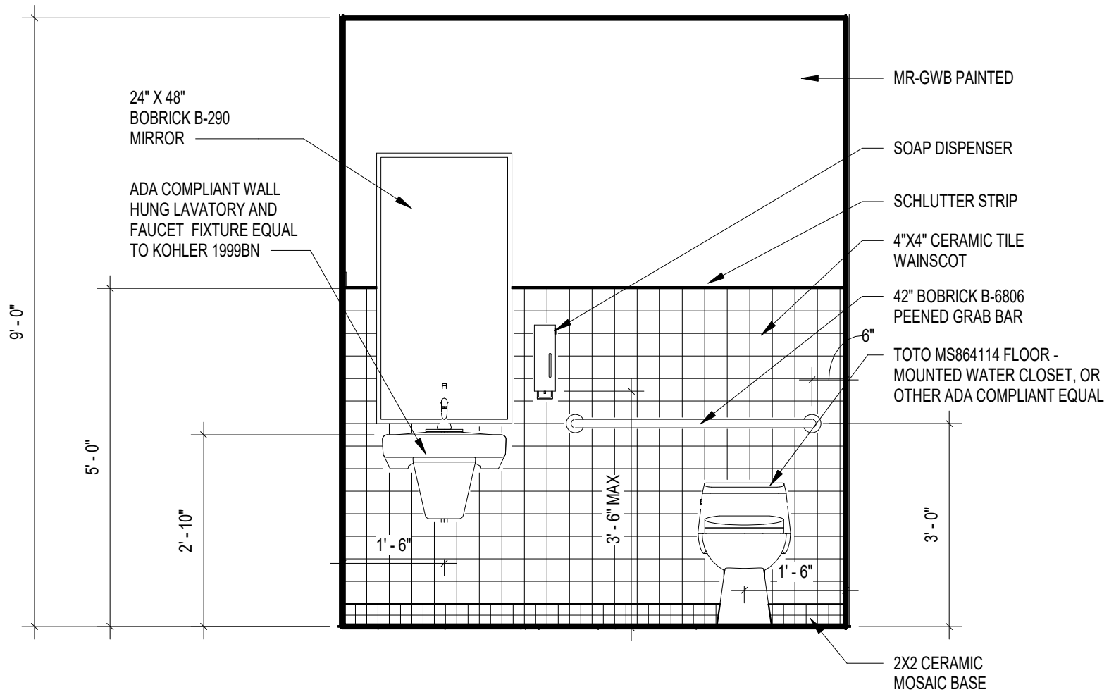
① TOILET - SOUTH -AMENDED PERMIT 1/2" = 1'-0"
